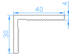
Abdeckwinkel 40x30 Code: 111.007
