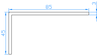
Abdeckwinkel 85x45 Code: 109.134
