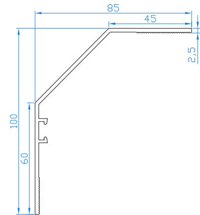
Abdeckwinkel 85x100 Code: 109.373
