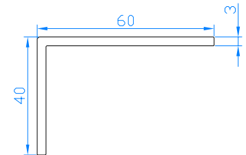
Abdeckwinkel 60x40 Code: 109.001
