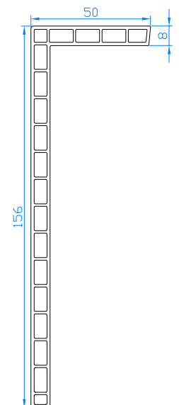
Abdeckwinkel 50x156 Code: 111.032
